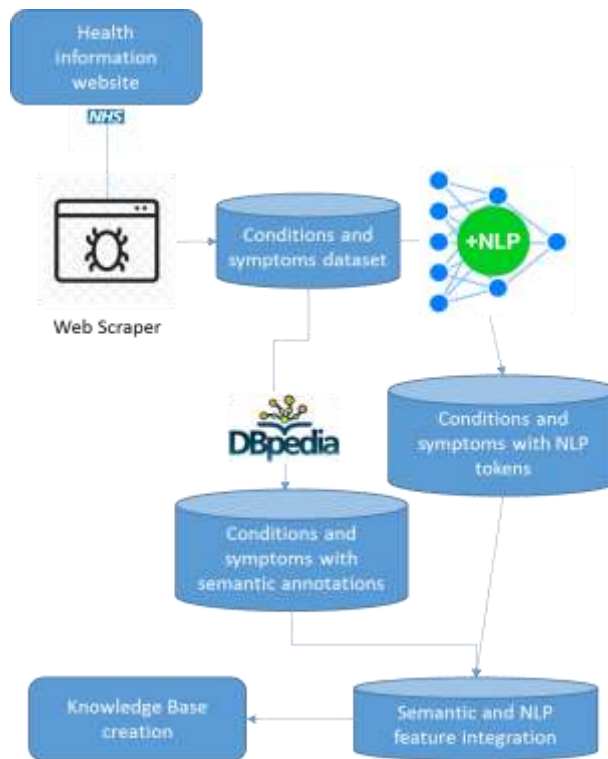
Fig. 1: Knowledge Graph creation process.
