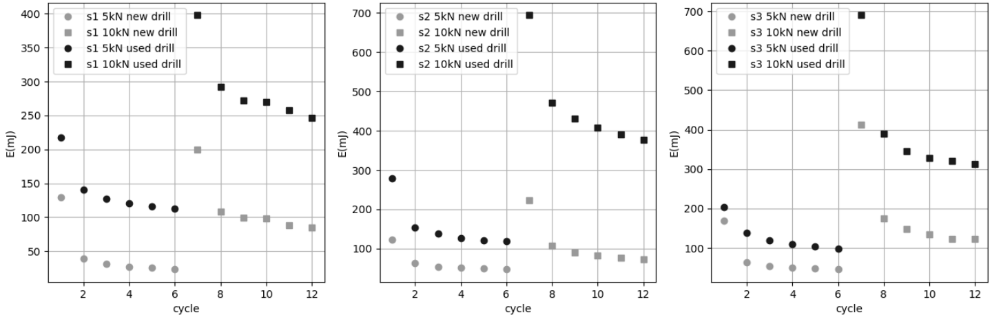
Fig. 5: Energy dissipation per cycle for all samples.
