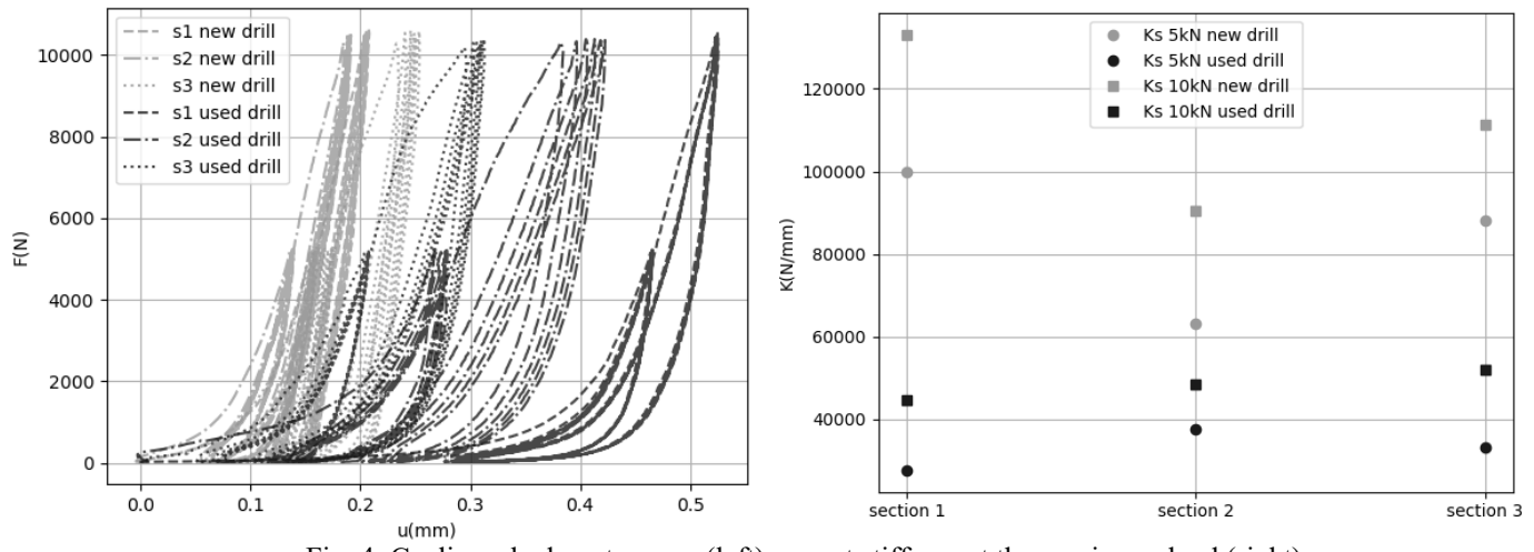
Fig. 4: Cyclic embedment curves (left), secant stiffness at the maximum load (right).
