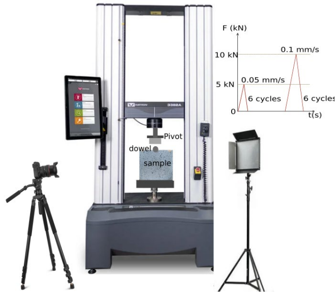
Fig. 2: Test set-up and loading.
