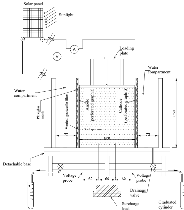
Figure 1. Elevation view of electrokinetic remediation cell (dimensions in mm)
