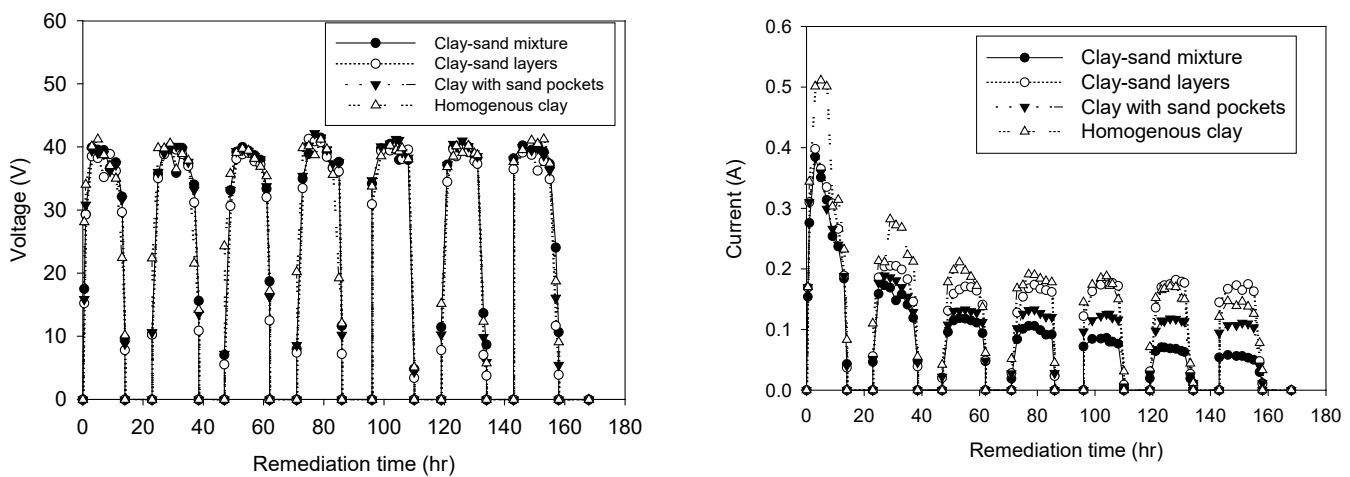
Figure 2. (a) Applied voltage and (b) Electric current
