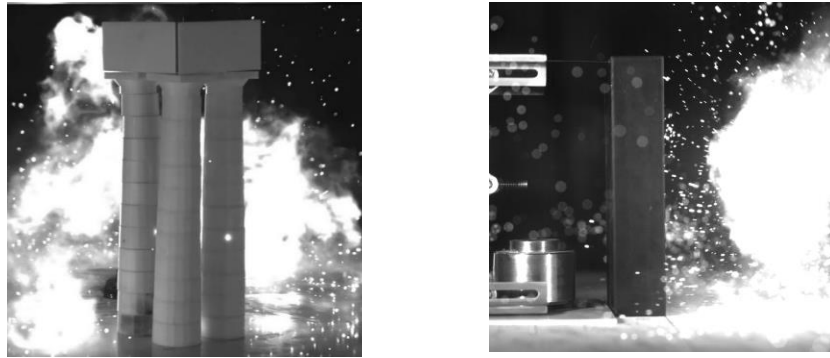
Fig. 5: Models (rocking structures) subjected to the fast-dynamic excitations arising from the denotation of an exploding wire.
