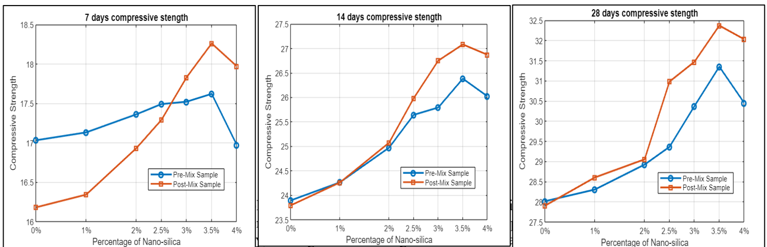
Figure 5: Compressive strength of pre-mix and post-mix samples for (a) 7 days, (b) 14 days and (c) 28 days
