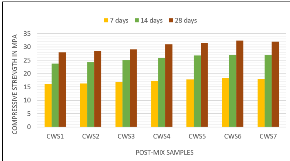
Figure 4: Post mix samples compressive strength for 7, 14, 28 days
