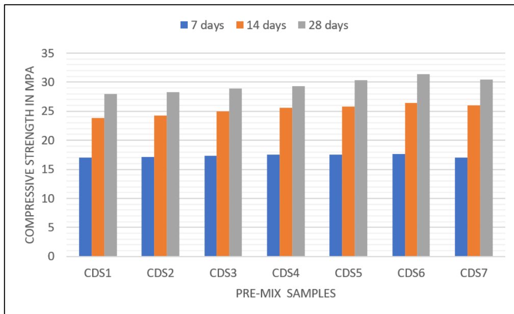
Figure 3: Pre mix samples compressive strength for 7, 14, 28 days
