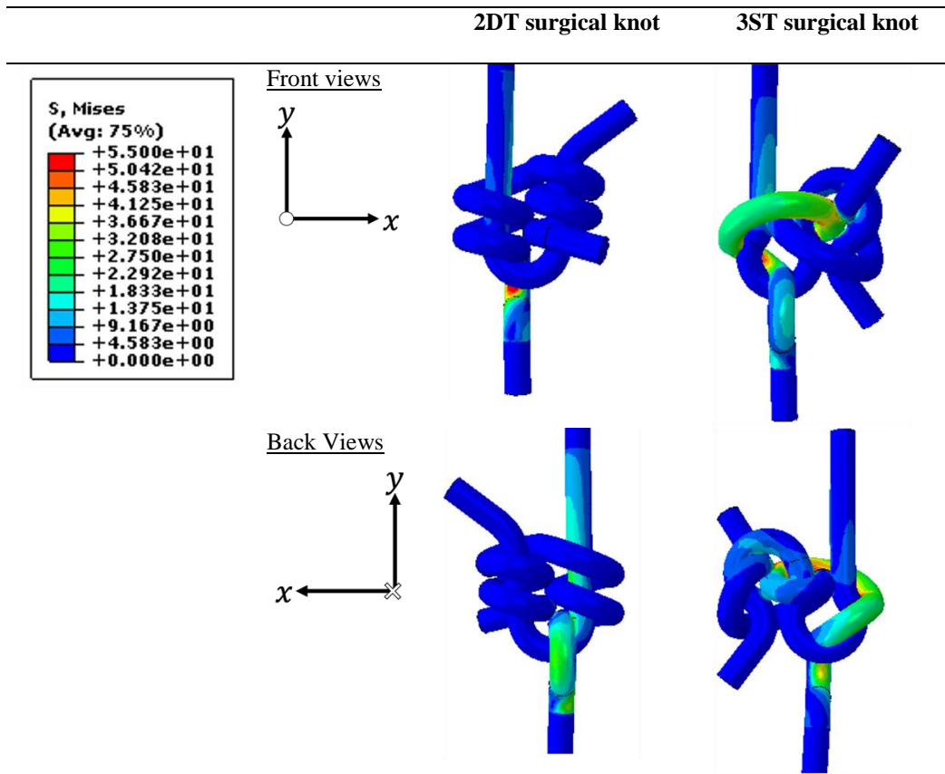
Fig. 4: Resultant von Mises Stresses in the two double throws (2DT) square surgical knot and the three single throws (3ST) surgical knot. Both the front and back views are shown of each configuration.
