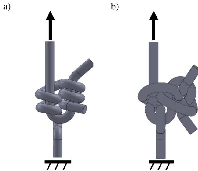
Fig. 3: 3D CAD models of the a) Two double throws surgical knot, and b) three single throws surgical knot. The bottom of each suture is fixed, and the top end of the suture is subjected to an applied load.
