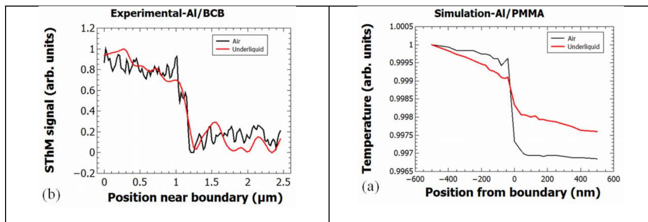
Fig. 5. (Left panel) Experimentally measured spatially resolved response of the iSThM probe compared to SThM response of the same probe in the air environment produced by scanning across the polymer – Al interface. (Right panel) FEA simulation of the same response.
