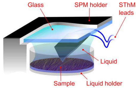
Fig. 3. Experiment setup of iSThM cell.
