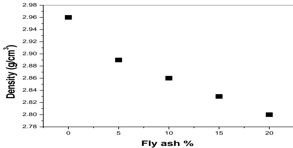
Fig. 6. Showing the effect of Fly ash percentage addition on the ratio 1:1
