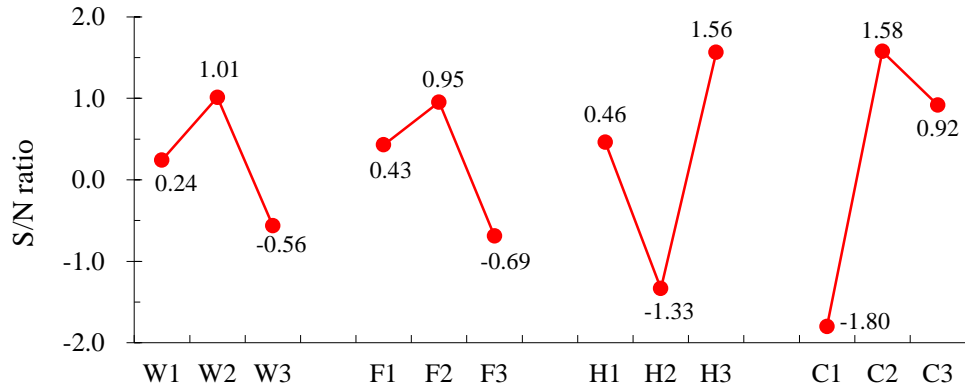
Fig. 2: The factor response diagram of S/N ratios for drilling time.
