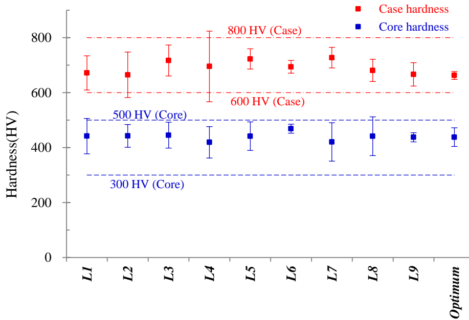
Fig. 3: The natural variation of the process (6S) for the case and core hardness.
