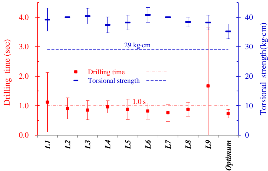
Fig. 4: The natural variation of the process (6S) for the torsional strength and drilling time.
