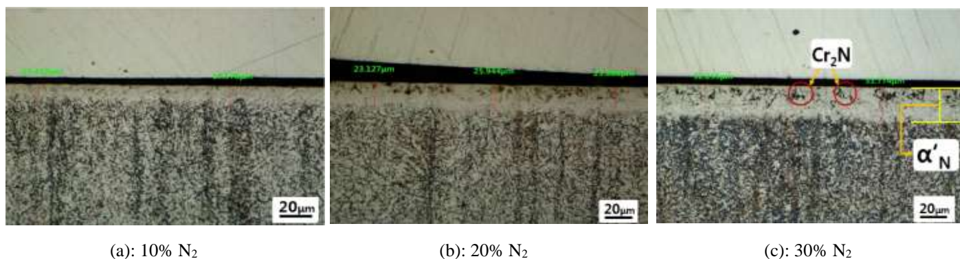
Fig. 4: AISI 420 samples for changing N 2 percentage at 400°C for 6h.
