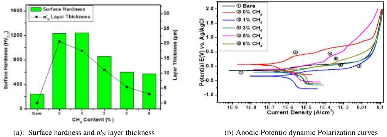
Fig. 9: AISI 420 samples for changing CH 4 percentage with 25% N 2 at 400°C for 6h.
