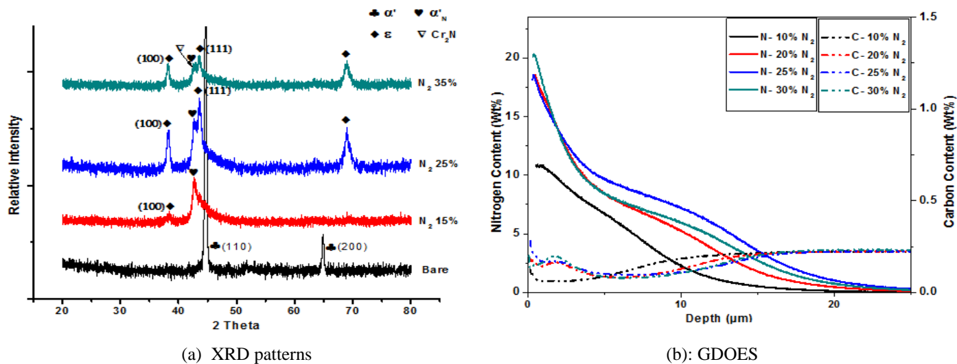
Fig. 4: AISI 420 samples for changing N 2 percentage at 400°C for 6h.
