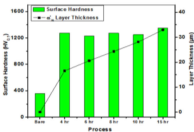
(a) Surface hardness and \alpha'_N layer thickness
