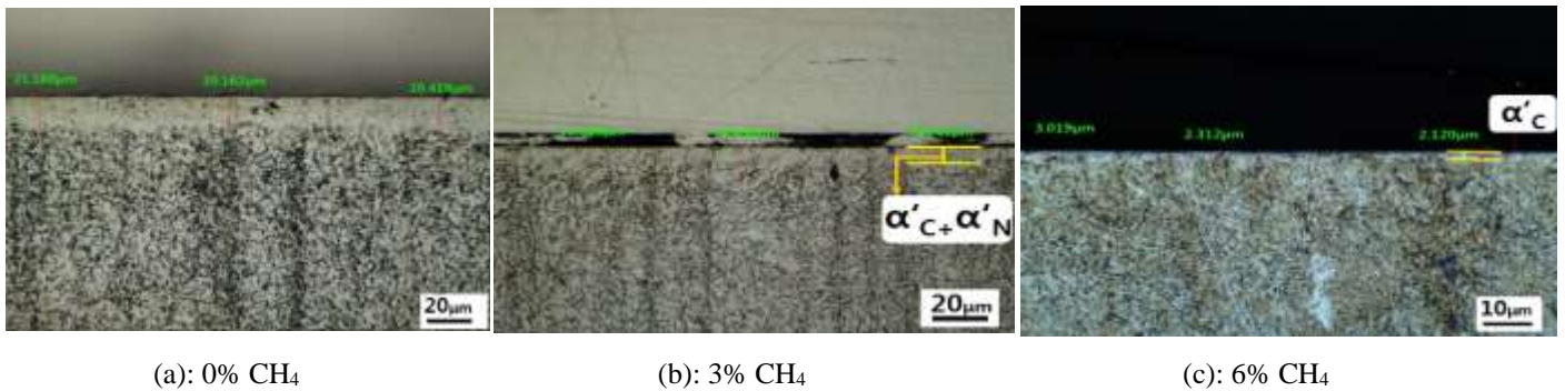
Fig. 8: Optical micrographs of AISI 420 samples for changing CH 4 percentage with 25% N 2 at 400°C for 6h.
