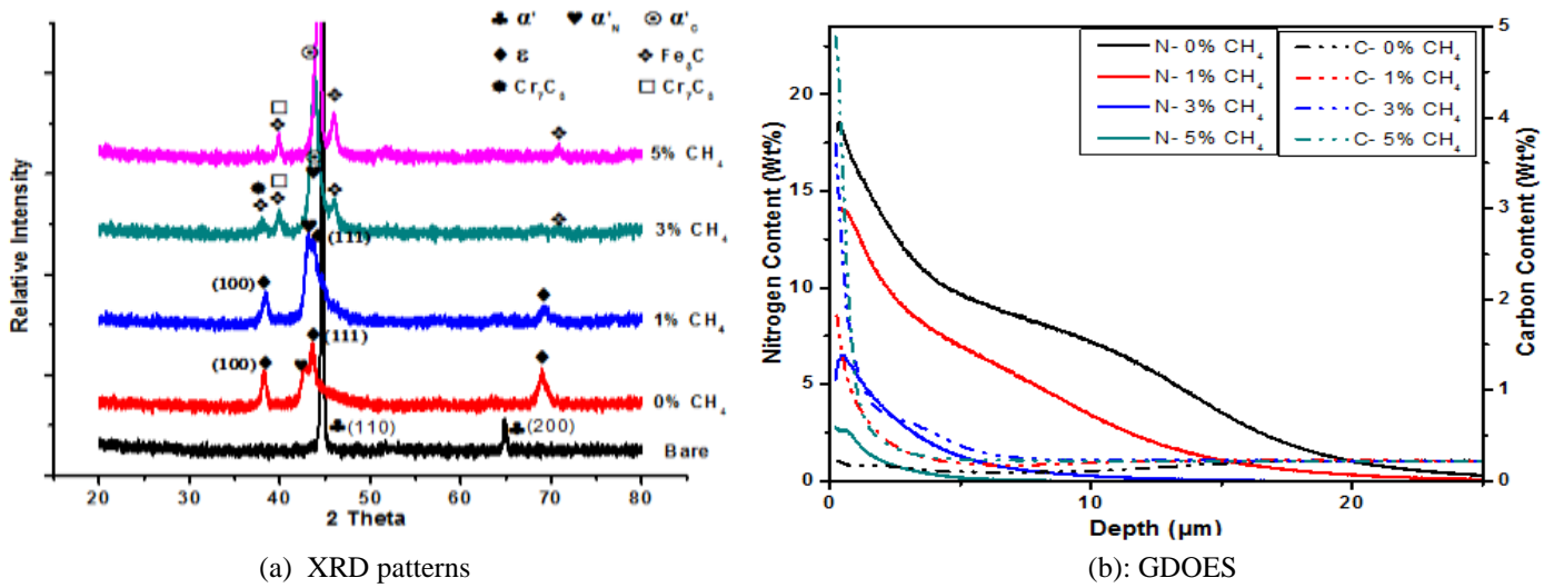
Fig. 7: AISI 420 samples for changing CH 4 percentage with 25% N 2 at 400°C for 6h.
