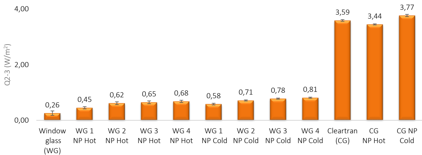
Fig. 6b: The comparison of the obtained heat flux for ZnS-SiO 2 NPs at 313 K
