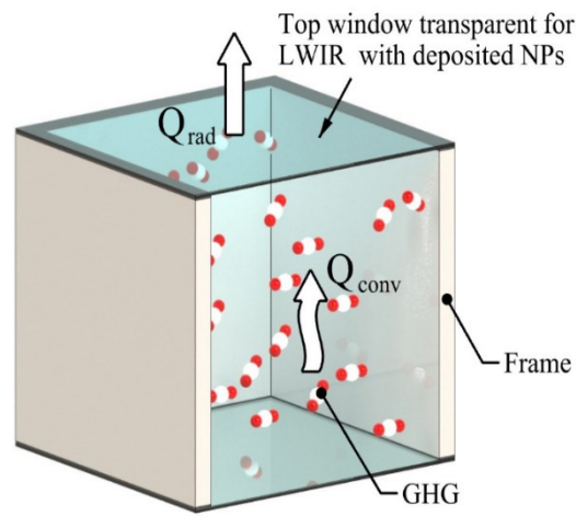
Fig. 2b: A skylight design with dispersed NPs on Cleartran®
