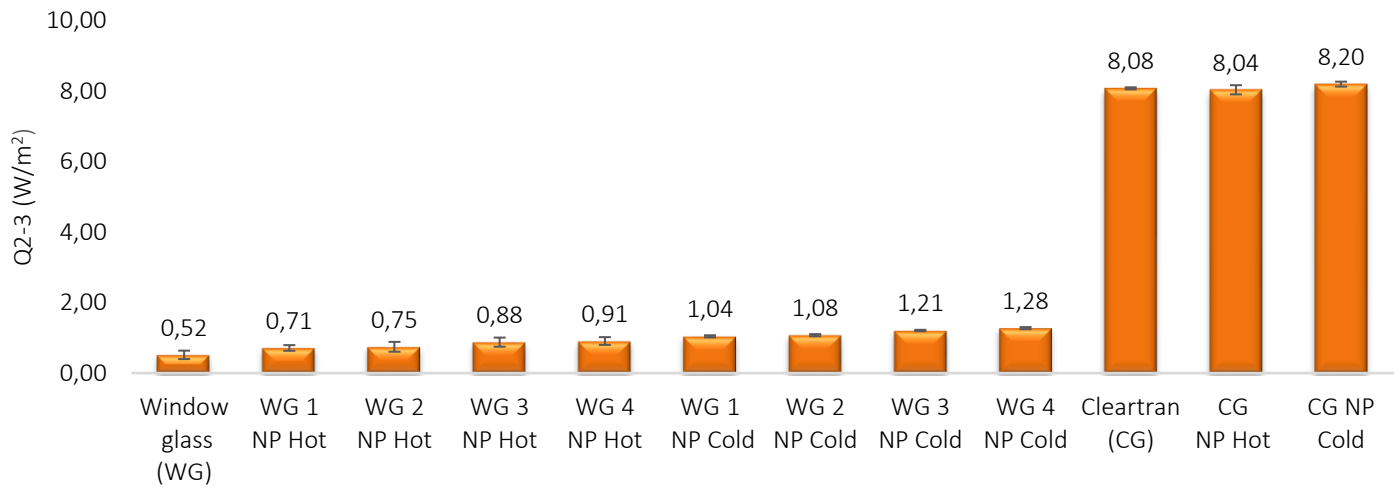
Fig. 7a: The comparison of the obtained heat flux for TiO 2 -SiO 2 NPs at 333 K
