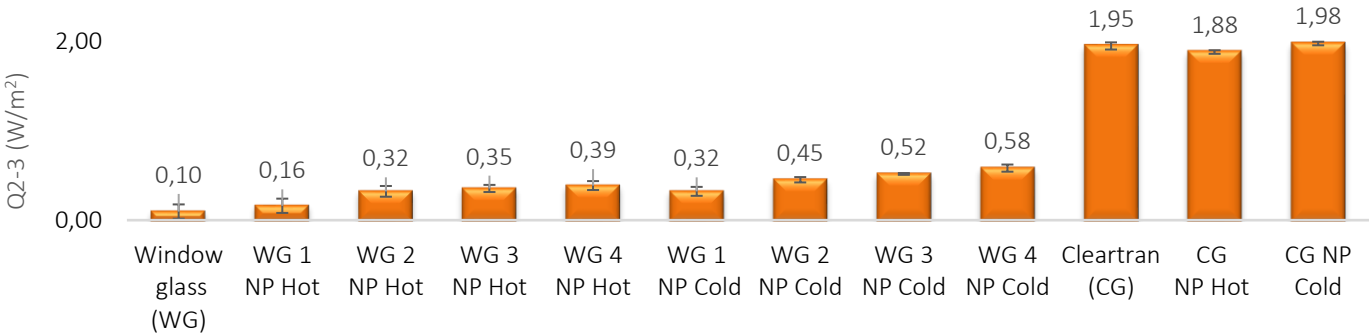
Fig. 5a: The comparison of the obtained heat flux for \text{TiO}_2\text{-SiO}_2 NPs at 303K
