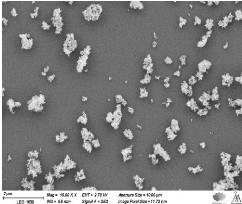
Fig. 4a: SEM images of \text{TiO}_2\text{-SiO}_2 NPs on glass substrate
