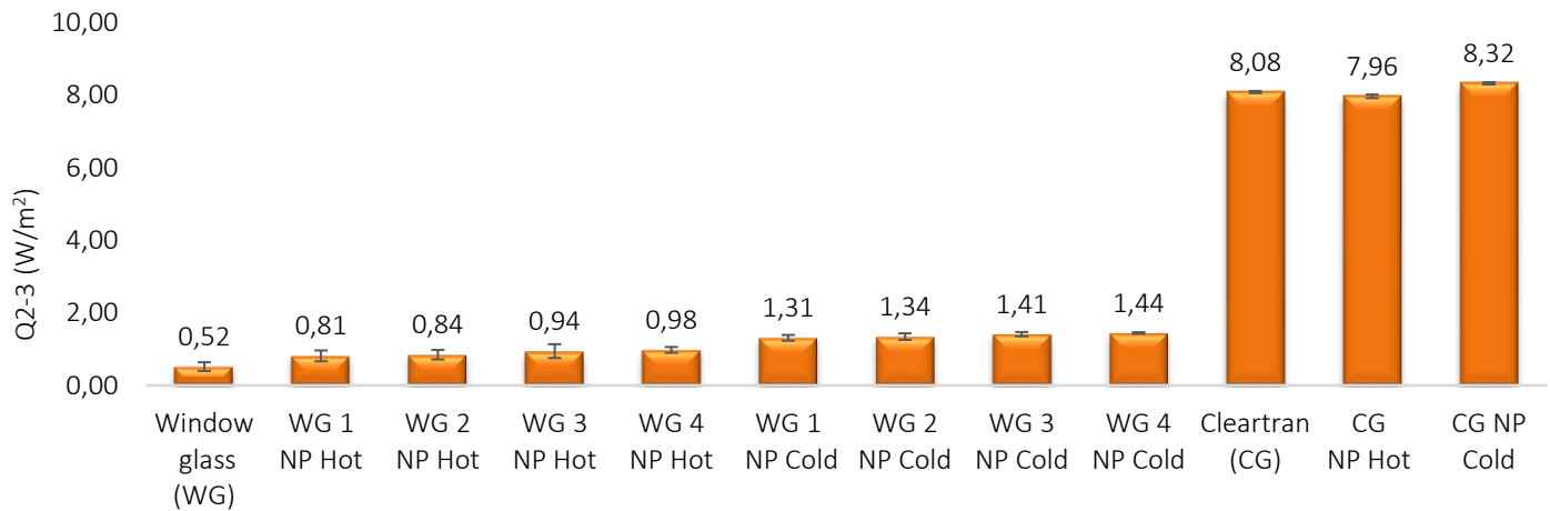
Fig. 7b: The comparison of the obtained heat flux for ZnS-SiO 2 NPs at 333 K
